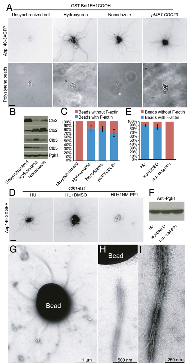
Fig. 1. Reconstitution of actin cables nucleated by Bni1 on polystyrene microspheres in yeast cytoplasmic extracts. (A) GST-Bni1 FH1-COOH-functionalized 2- \mu\text{m} microspheres were added to different cytoplasmic extracts generated from yeast cells expressing Abp140-3×GFP. Extracts prepared from HU-, nocodazole-, and pMET-CDC20 -arrested cells, but not from unsynchronized cells, support actin cable assembly. Polystyrene beads are shown by transillumination. (B) The percentage of beads with or without actin cables for the reactions in A, including unsynchronized ( n = 10 individual experiments) and HU- ( n = 9 ), nocodazole- ( n = 4 ), and pMET-CDC20 -arrested cells ( n = 4 ). (C) Cyclin levels were determined by Western blotting of extracts from unsynchronized and HU- and nocodazole-arrested cells. Pgk1 was used as a loading control. (D) Inhibition of Cdk1 activity using 1NM-PP1 on HU-arrested cdk1-as1 cells before extract preparation blocks actin cable formation by GST-Bni1 FH1-COOH-coated beads. 1NM-PP1 at a final concentration of 20 \mu\text{M} was added for 30 min before sample preparation. (E) The percentage of beads with or without actin cables for reactions in D ( n = 3 ). (F) The protein concentrations for cytoplasmic extracts used for actin reconstitution in D are compared by anti-Pgk1 Western blot. (Scale bars, 5 \mu\text{m} .) (G–I) Actin cables were assembled from GST-Bni1 FH1-COOH-functionalized beads in cell extracts derived from HU-arrested cells. Polymerized F-actin was negatively stained and visualized by EM. (G) Actin cables emanating from polystyrene beads, viewed at low magnification by negative-staining EM. (H and I) High-magnification images showing actin filament bundles.
